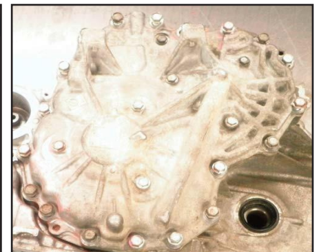
Using loctite 509 sealer, install end cover onto the main case. Torque 35 ft lbs
