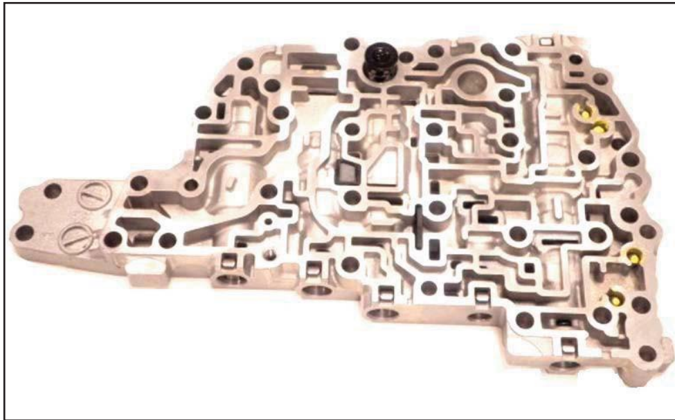
Center valve body, check valve and screens installed
