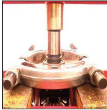
Remove both differential side bearings.
