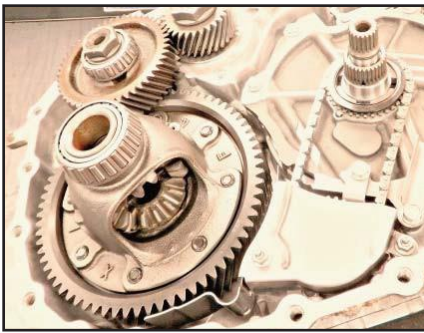
Install differential and transfer gears
