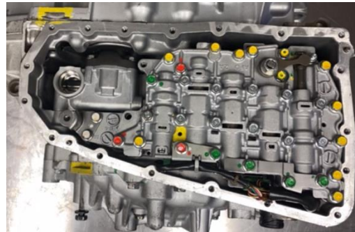
Install wiring harness bracket
