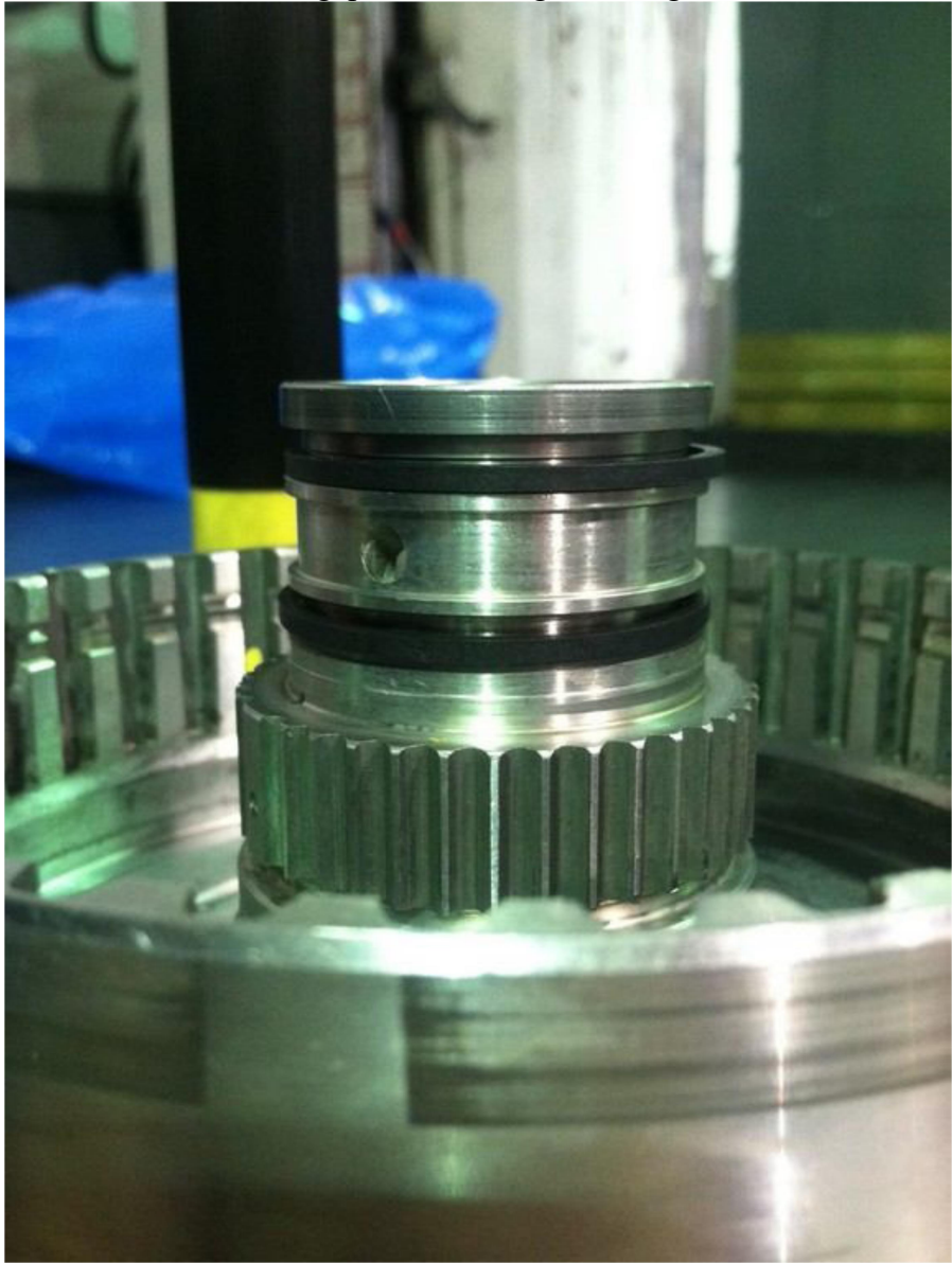
Bad drum – Too much gap between rings and ring lands.
